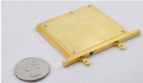
Millimeter Wave Phased Array Modules
